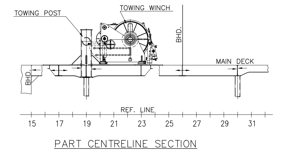
PART CENTRELINE SECTION
