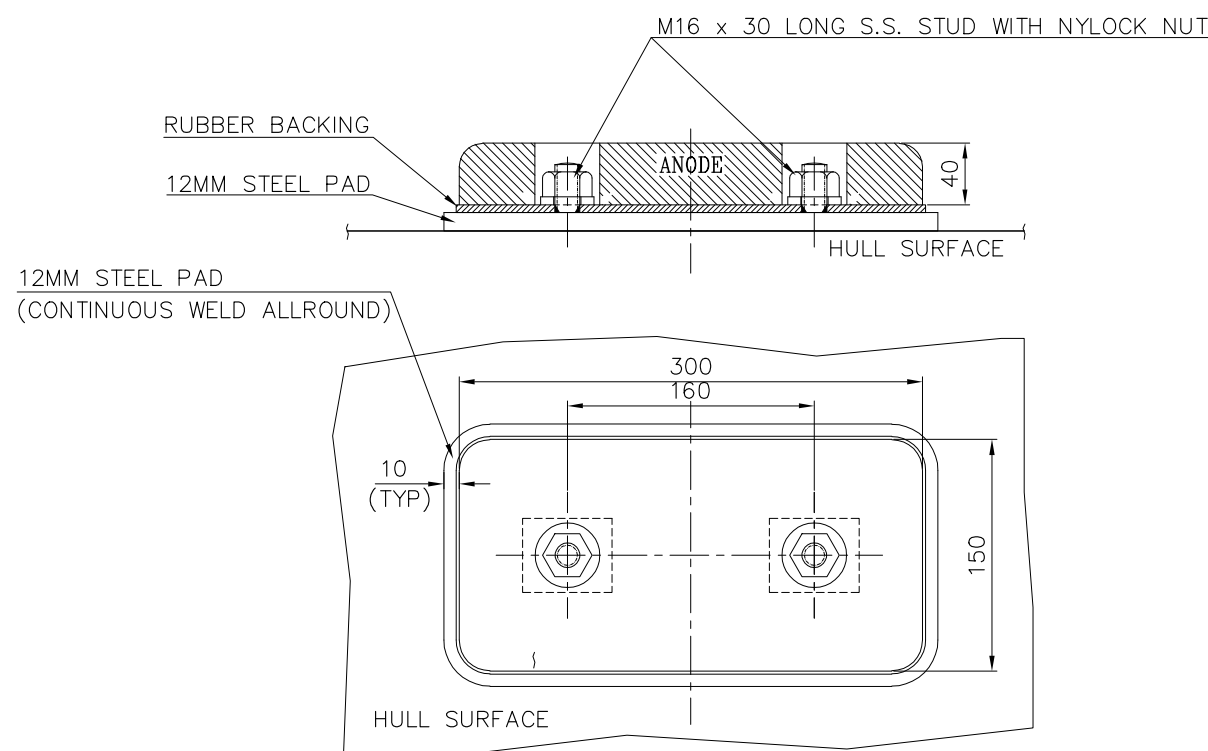
TYPICAL DETAIL OF ANODES (SCALE 1:5)
