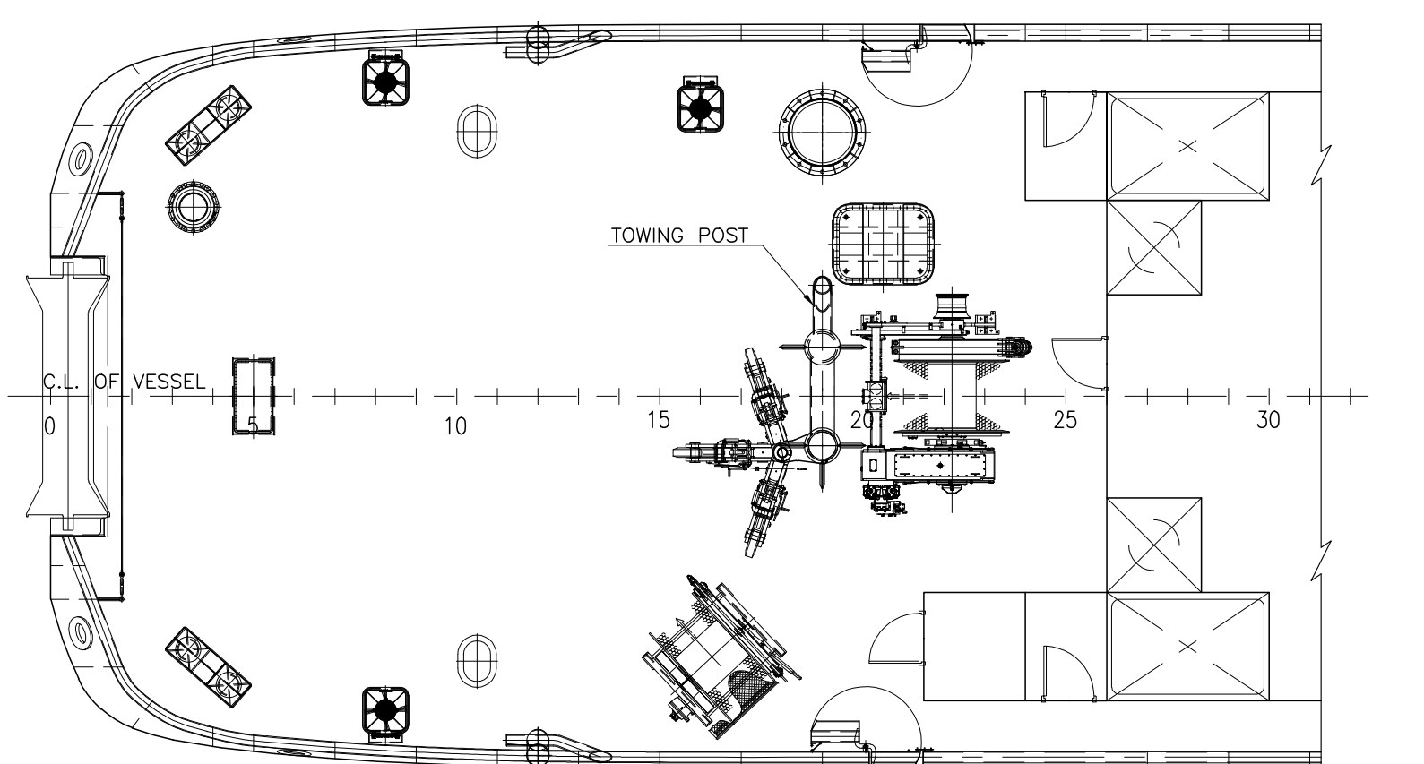
PART MAIN DECK PLAN
