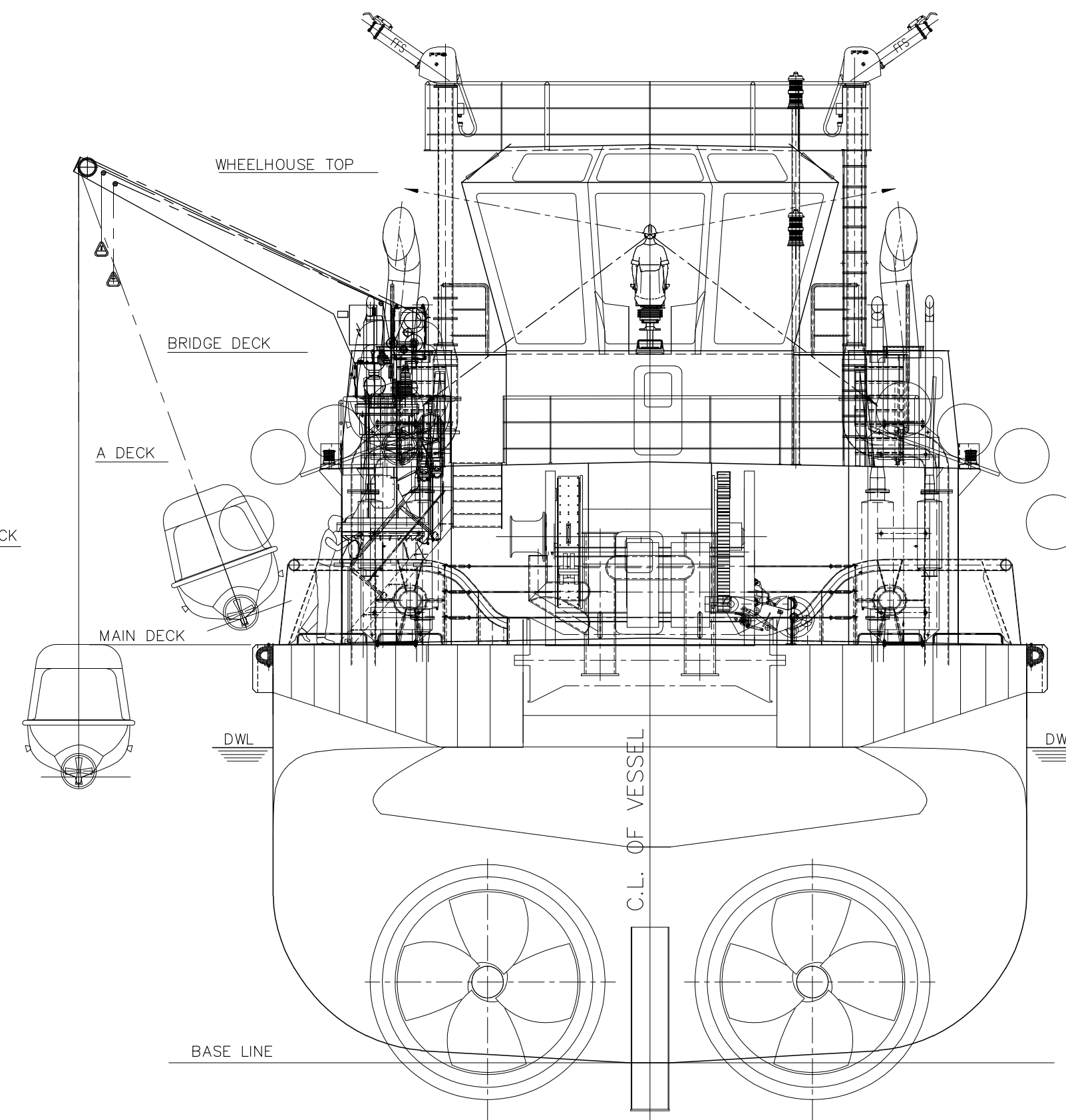
AFT VIEW
